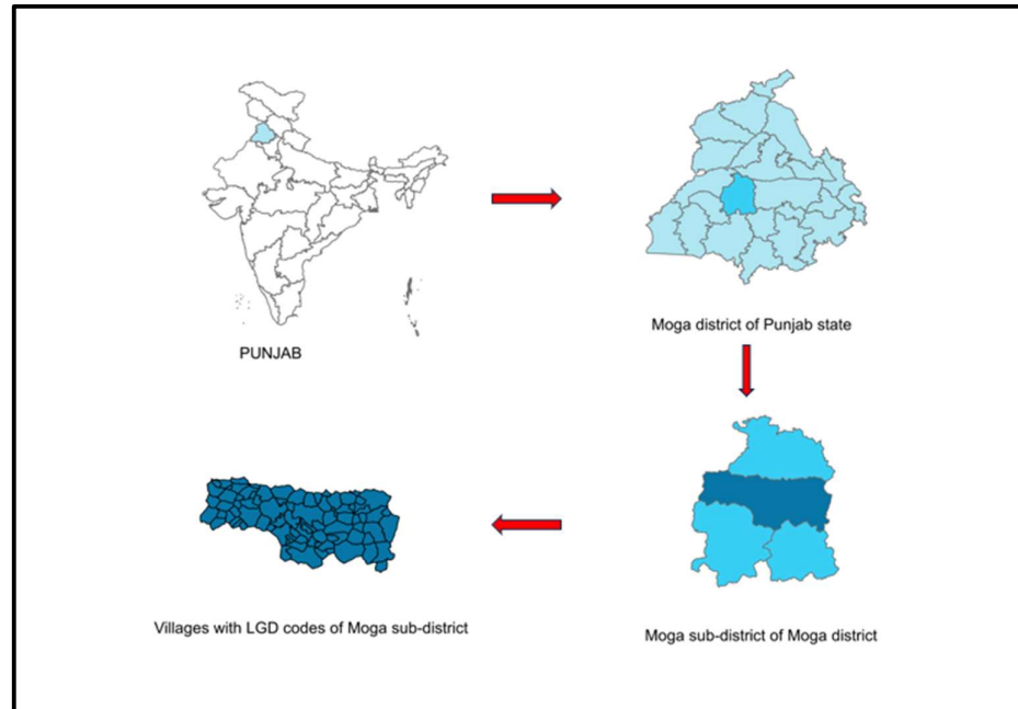
Fig 2: Administrative Boundaries: From International boundary to Village boundary
