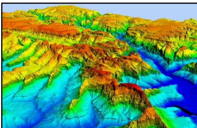
Fig 3: Digital Elevation Model
